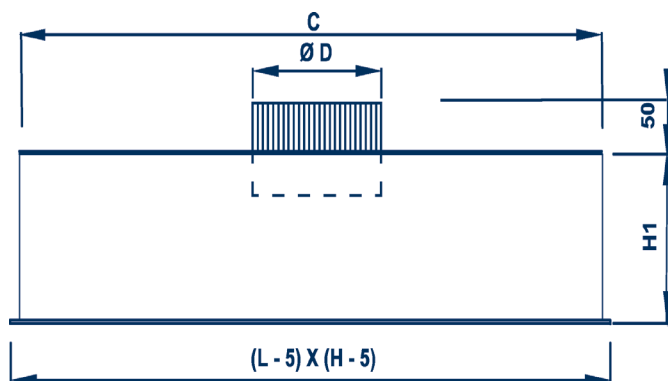
DHFP + PL/V (plenum vertical)
